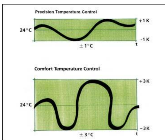
Temperature Control Comparison
