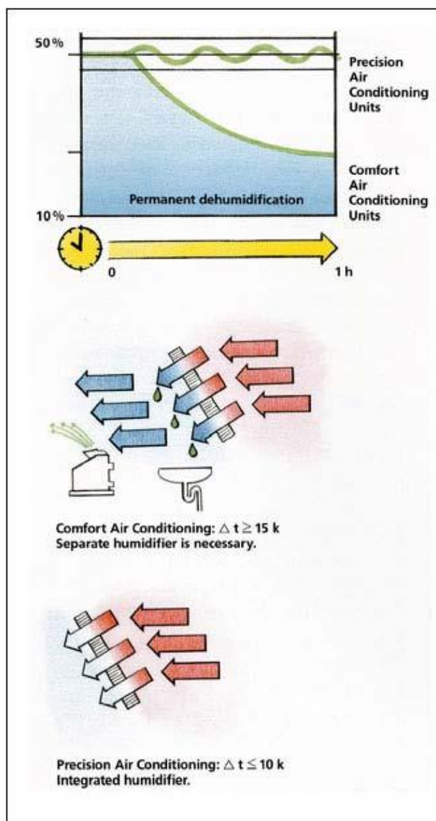
Humidity Control Comparison
