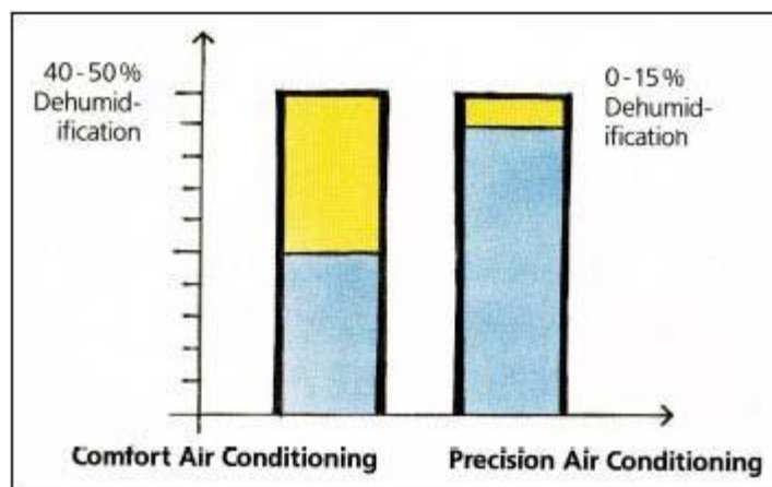
Dehumidification Effect Comparison
